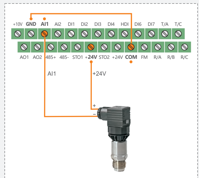
Wiring diagram of 24V pressure sensor
